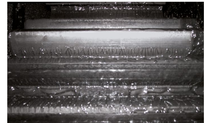
Flanks of the kiln drive after 7 days running-in with Berulit EL 420
